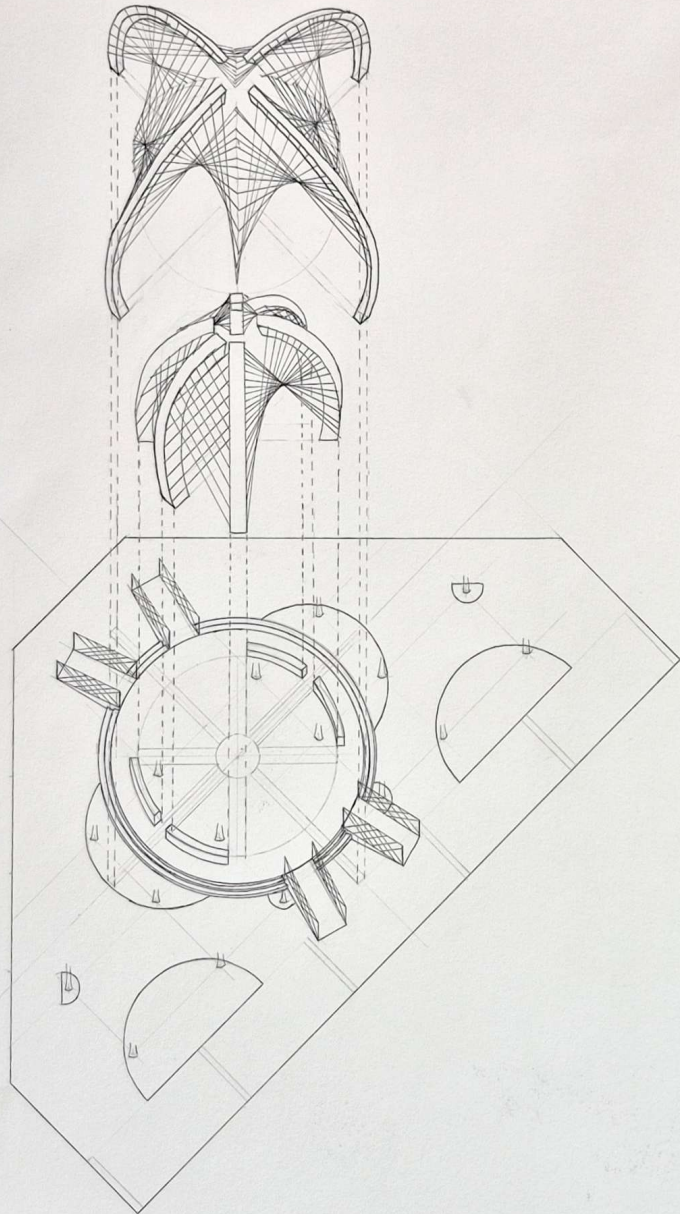
EXPLODED AXONOMETRIC
